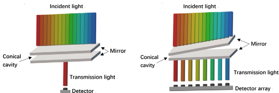
(a) 可调谐法布里-珀罗滤光片分光示意图 (a) Schematic diagram of tunable Fabry-Perot filter (b) 线性滤光片分光示意图 (b) Schematic diagram of linear filter splitting
